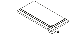
* step tread "L" corner inox nez de marche "L" angle inox ecke stufenplatte "L" inox degrau "L" canto inox
