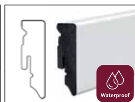
Stick-on skirtings PS foam, waterproof, sui- table for damp rooms, 15x50 mm (cube) 3 Length: 240 cm
