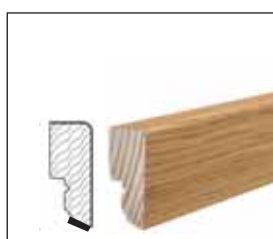
Skirtings Solid wood core without recess for clips with white insulation strip
