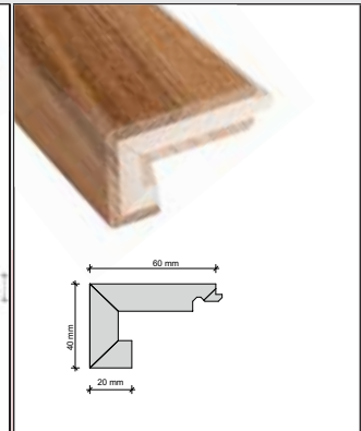
Stair nosing, angled
