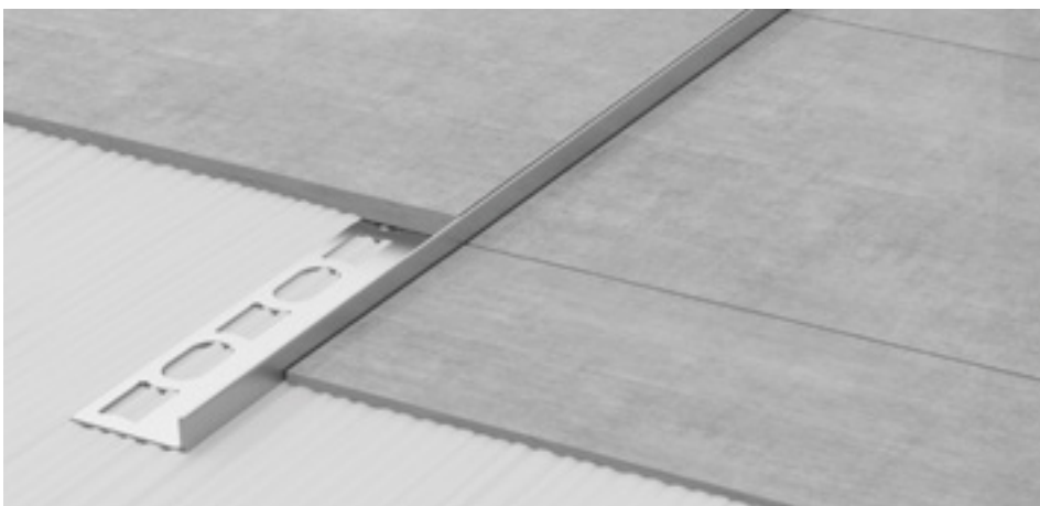
GPS3/SX/10 brushed stainless steel AISI 304 DIN 1.4301
