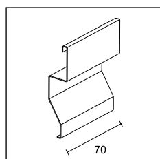
CPGV/N/ /G single piece
