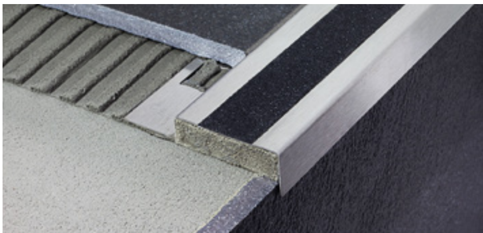
SIX/10 brushed stainless steel AISI 304 - DIN 1.4301 + black slip-resistant 25 mm
