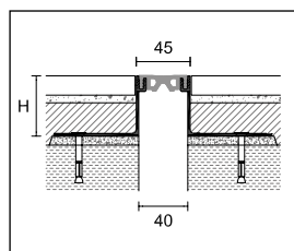
PBE/40 smooth plasticised PVC
