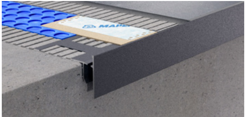
CPQV/50/10 ancient grey colour-coated aluminium
