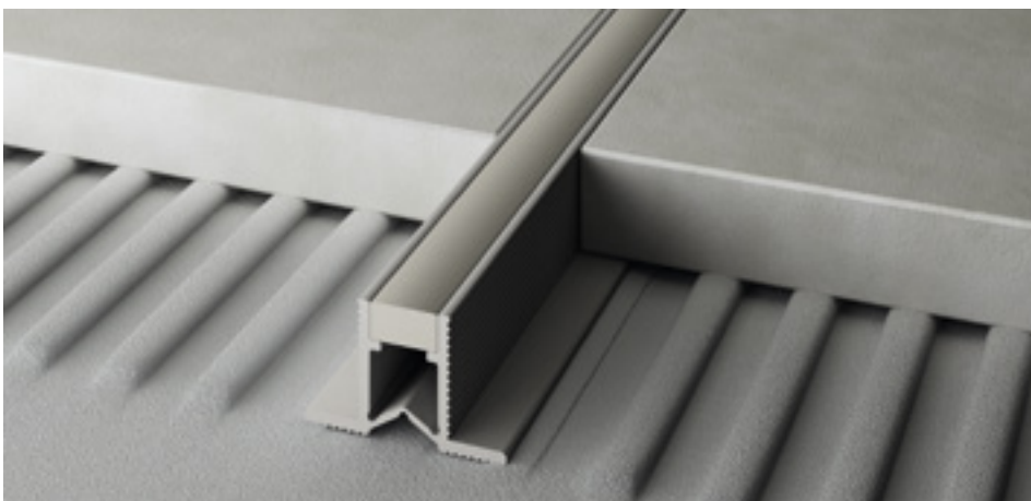
NE/10 co-extruded PVC grey + grey RAL 7035
