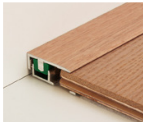
S/9/SF aluminium covered with Alchrom® Plus film
