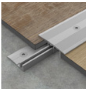
FIX/J/30 silver anodised aluminium
