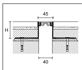
PBE/40 striated plasticised PVC
