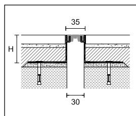
PBE/30 striated plasticised PVC
