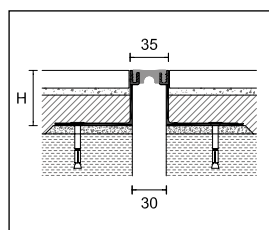
PBE/30 smooth plasticised PVC
