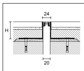
PBE/20 striated plasticised PVC
