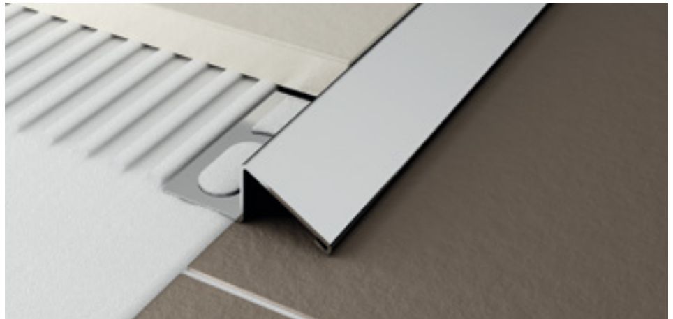
PNI/10 polished stainless steel AISI 304 DIN 1.4301
