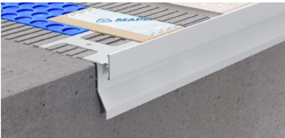
CPGV/55/10 stone white colour-coated aluminium
