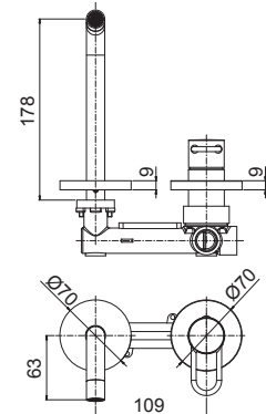
JK 105-104-106CR70 Miscelatore incasso con bocca erogazione a muro 178 mm / 123 mm / 248 mm corpo incasso incluso Concealed wash basin mixer with wall spout 178 mm / 123 mm / 248 mm concealed body included
