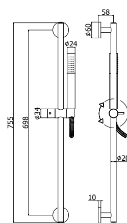
ZSAL 135NO LIFE Saliscendi Life con doccia (monogetto) in metallo Life sliding rail with (single-spray) metal hand-shower
