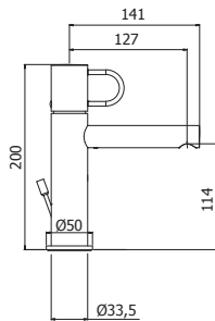
JK 071-071K-075CR Miscelatore lavabo con/senza scarico, con scarico Clic-Clac Wash basin mixer with/without pop up waste, with Clic-Clac press top waste
