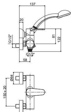
ND 168-168DCR Miscelatore doccia con/ senza set doccia Wall mounted shower mixer with/ without shower set
