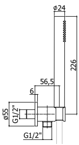
ZDUP 094CR-CRAG TONDO Set doccia incasso tondo con presa acqua incorporata / con flexibile PVC Round concealed shower set with build-in water inlet / with PVC flex
