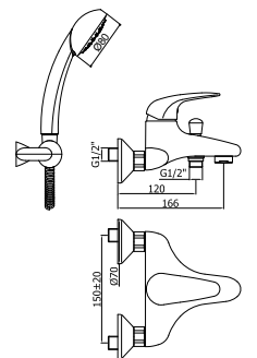
DU 022-023-024-026CR Miscelatore vasca con/ senza set doccia, con supporto a muro fisso ABS, con supporto Smart Bath/shower mixer with/ without shower set, with ABS fixed wall bracket, with Smart bracket
