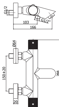
JOQ 022-023CR Miscelatore termostatico vasca/doccia attacco 1/2" con/ senza set doccia Thermostatic bath/shower mixer 1/2" connection with/ without shower kit
