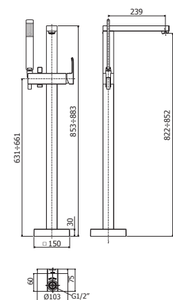
ELBOX 033CR Miscelatore vasca/doccia a pavimento Free-standing bath/shower mixer
