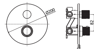
JOQ 018CR Miscelatore termostatico incasso 2 uscite corpo incasso incluso Concealed thermostatic 2 outlets concealed body included
