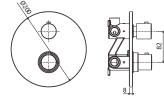
LIQ 019CR Miscelatore termostatico incasso 3 uscite corpo incasso incluso Concealed thermostatic 3 outlets concealed body included
