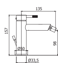
JL 131-131K-135CR Miscelatore bidet con/senza scarico, con scarico Clic-Clac Bidet mixer with/without pop up waste, with Clic-Clac press top waste
