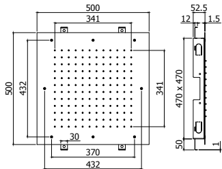
ZSOF 301CR BOSTON Soffione ad incasso "Quadro" in metallo, anticalcare - 500x500 mm "Square" concealed ceiling metal shower head, antiscaling system - 500x500 mm
