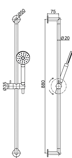
ZSAL 215AC INOX SOFT Saliscendi INOX con doccia e supporto scorrevole INOX sliding rail with hand-shower and slider bracket
