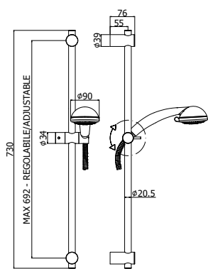
ZSAL 119CR ROYAL Saliscendi Royal con doccia (4 getti) in ABS Royal sliding rail with (4-spray functions) ABS hand-shower
