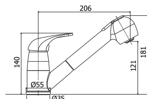
APM3 183CR Miscelatore lavello con doccia estraibile (2 getti) e canna tubo orientabile One-hole sink mixer with pull-out hand-shower (two-spray) and swivelling spout
