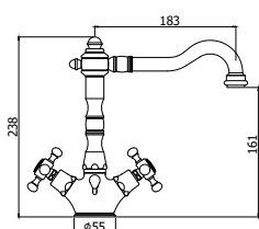
FBLV 071-075CR Monoforo lavabo con/ senza scarico One-hole wash basin mixer with/ without pop up waste
