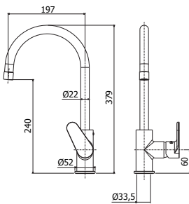
GR 180CR Miscelatore lavello monoforo con canna tubo orientabile One-hole sink mixer with tube swivelling spout
