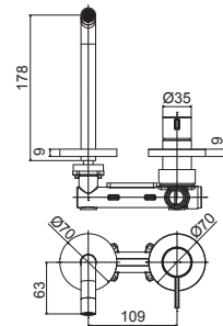
FOX 105-104-106CR 70 Miscelatore incasso con bocca erogazione a muro 178 mm / 123 mm / 248 mm corpo incasso incluso Concealed wash basin mixer with wall spout 178 mm / 123 mm / 248 mm concealed body included
