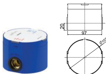
PBOX 005 Set incasso universale per miscelatori VASCA/LAVABO FREESTANDING Universal Concealed Box for Free-standing bath/shower mixer * Da abbinare solo con JK BOX031 - JK BOX032 To be completed only with JK BOX031 - JK BOX032
