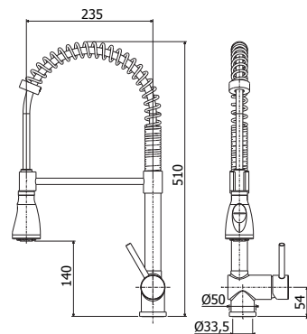
SK 177CR Miscelatore lavello "Professional" con doccetta bombata 2 getti One-hole sink mixer "Professional" with two-spray round hand-shower
