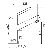
BI 071-071K-075CR Miscelatore lavabo con/ senza scarico, con scarico Clic-Clac Wash basin mixer with/ without pop up waste, with Clic-Clac press top waste
