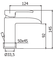
LES 061-061K-065CR Miscelatore lavabo a cascata con/senza scarico, con scarico Clic-Clac Waterfall basin mixer with/without pop up waste, with Clic-Clac press top waste
