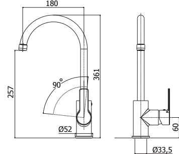
RED 181CR Miscelatore lavello monoforo con canna small orientabile One-hole sink mixer with small swivelling spout
