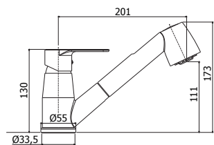
LM 183CR Miscelatore lavello con doccia estraibile (2 getti) e canna tubo orientabile One-hole sink mixer with pull-out hand-shower (two-spray) and swivelling spout
