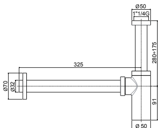
ZACC 526AC INOX Sifone a bottiglia tondo Inox con attacco 1"1/4" Round Inox bottle trap with 1"1/4" connection
