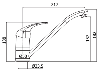
ND 182TCR Miscelatore lavello monoforo con canna tubo orientabile One-hole sink mixer with tube swivelling spout
