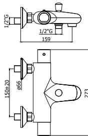
EQS 022-023CRNEW Miscelatore termostatico vasca/doccia attacco 1/2" con senza set doccia Thermostatic bath/shower mixer 1/2" connection with without shower kit
