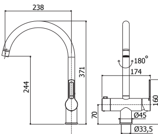
RIN 184CR Miscelatore lavello monoforo alto con canna orientabile e attacco lavastoviglie Tall one-hole sink mixer with swivelling spout and dish-washer connection
