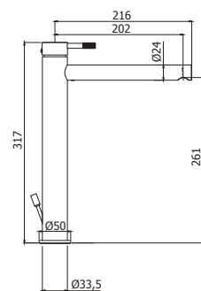
JL 081-081K-085CR Miscelatore lavabo prolungato con/senza scarico, con scarico Clic-Clac Tall wash basin mixer with/without pop up waste, with Clic-Clac press top waste
