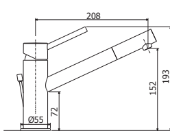
BI 081-085CR Miscelatore lavabo canna lunga con/ senza scarico Wash basin mixer with long spout with/ without pop up waste
