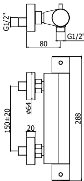
LIQ 468CR COLD TOUCH Miscelatore termostatico doccia attacco 1/2" senza set doccia Thermostatic shower mixer 1/2" connection without shower kit
