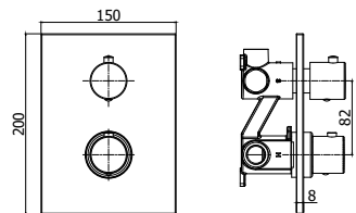
LIQ 519CR Miscelatore termostatico incasso 3 usci- te corpo incasso incluso Concealed thermostatic 3 outlets concealed body included
