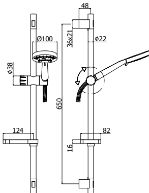
ZSAL 206CR LUNA Saliscendi Luna con doccia (3 getti) in ABS Luna sliding rail with (3-spray functions) ABS hand-shower
