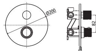
JOQ 019CR Miscelatore termostatico incasso 3 usci- te corpo incasso incluso Concealed thermostatic 3 outlets concealed body included
