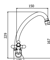
IRV 077-078CR Monoforo lavabo con bocca orientabile con/senza scarico One-hole wash basin mixer with swivelling spout with/without pop up waste
