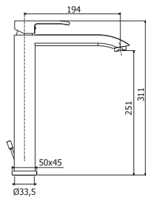
LES 081-081K-085CR Miscelatore lavabo prolungato, con/senza scarico, con scarico Clic-Clac Tall wash basin mixer with/without pop up waste, with Clic-Clac press top waste
