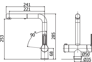
RIN 295CR - MET (3VIE) Miscelatore lavello monoforo con doccia in metallo e 3° ingresso per acqua depurata One-hole sink mixer with metal pull out hand-shower and 3rd inlet for purified water
