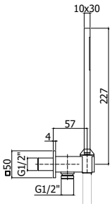
ZDUP 095CR-CRAG QUADRO Set doccia incasso quadro con presa acqua incorporata / con flexibile PVC Square concealed shower set with build-in water inlet / with PVC flex
