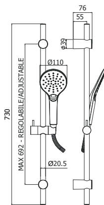
ZSAL 210CR SOFIA Saliscendi Sofia con doccia (2 getti) in ABS Sofia sliding rail with (2-spray functions) ABS hand-shower
