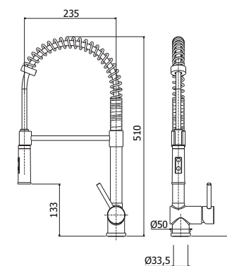
SK 179CR Miscelatore lavello "Professional" con doccetta ABS Minimal 2 getti One-hole sink mixer "Professional" with two-spray ABS Minimal hand-shower
