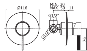
FOX 010CR Miscelatore incasso doccia corpo incasso incluso Concealed shower mixer concealed body included
