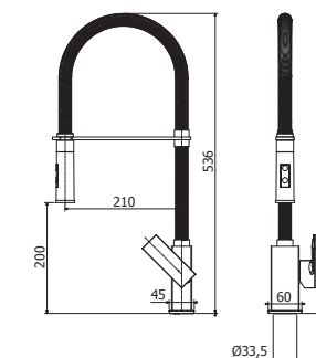
EL 179CR Miscelatore lavello "Professional" con doccia estraibile (2 getti) e canna orientabile One-hole "Professional" sink mixer with pull-out hand-shower (two-spray) and swivelling spout
