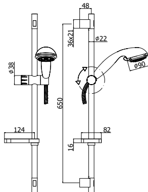
ZSAL 121CR QUEEN Saliscendi Queen con doccia (4 getti) in ABS Queen sliding rail with (4-spray functions) ABS hand-shower
