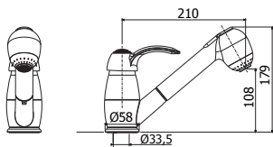
FA 183CR Miscelatore lavello con doccia estraibile (2 getti) e canna orientabile One-hole sink mixer with pull-out hand-shower (two-spray) and swivelling spout
