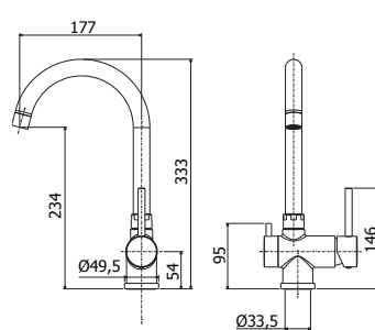
SK 184CR Miscelatore lavello monoforo con canna orientabile e attacco lavastoviglie One-hole sink mixer with swivelling spout and dish-washer machine connection
