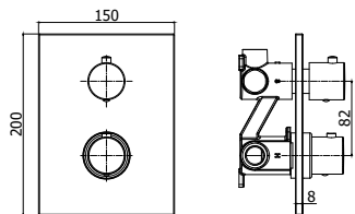
LIQ 513CR Miscelatore termostatico incasso doccia corpo incasso incluso Concealed thermostatic shower mixer concealed body included
