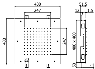
ZSOF 300CR NEW YORK Soffione ad incasso "Quadro" in metallo, anticalcare - 430x430 mm "Square" concealed ceiling metal shower head, antiscaling system - 430x430 mm
