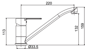
RED 182TCR Miscelatore lavello monoforo con canna orientabile One-hole sink mixer with swivelling spout
