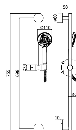
ZSAL 146C RAG LIFE GINEVRA - VRA Saliscendi Life Ginevra con doccia (3 getti) in ABS Life Ginevra sliding rail with (3-spray functions) ABS hand-shower
