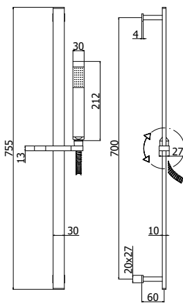
ZSAL 145CRAG CITY Saliscendi City con doccia (monogetto) in metallo City sliding rail with (single-spray) metal hand-shower
