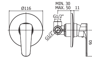
SY 010CR Miscelatore incasso doccia corpo incasso incluso Concealed shower mixer concealed body included
