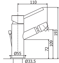
BI 131-131K-135CR Miscelatore bidet con/ senza scarico, con scarico Clic-Clac Bidet mixer with/ without pop up waste, with Clic-Clac press top waste
