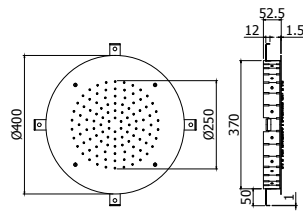
ZSOF 303CR LOS ANGELES Soffione ad incasso "Tondo" in metallo, anticalcare - Ø 400 mm "Round" concealed ceiling metal shower head, antiscaling system - Ø 400 mm
