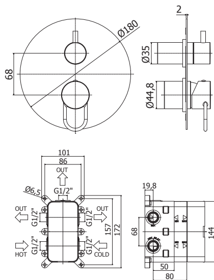
PBOX 003/004 Set incasso universale per miscelatori doccia 2 o 3 vie Universal Concealed Box for mixers 2 or 3 oulet
