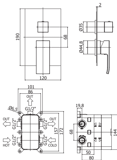
PBOX 003/004 Set incasso universale per miscelatori doccia 2 o 3 vie Universal Concealed Box for mixers 2 or 3 outlet
