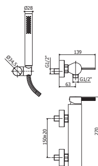
FOX 168-168DCR Miscelatore doccia attacco 1/2" con/ senza set doccia Shower mixer 1/2" connection with/ without shower set
