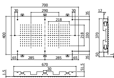
ZSOF 302CR MIAMI Soffione ad incasso " Rettangolare" in metallo, anticalcare - 700x400 mm "Rectangular" concealed ceiling metal shower head, antiscaling system - 700x400 mm
