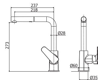
SY 285CR Miscelatore lavello monoforo con doccia estraibile (2 getti) e canna tonda orientabile One-hole sink mixer with pull-out hand- shower (two-spray) and round swivelling spout
