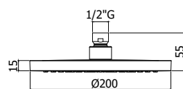
ZSOF 115CR PANDA Soffione "Panda" in ABS, anticalcare Ø 200 mm "Panda" ABS shower head, antiscala system Ø 200 mm
