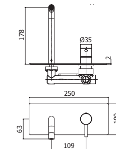
LIG 105-104-106CR Miscelatore incasso con bocca erogazione a muro 178 mm / 123 mm / 248 mm corpo incasso incluso Concealed wash basin mixer with wall spout 178 mm / 123 mm / 248 mm concealed body included
