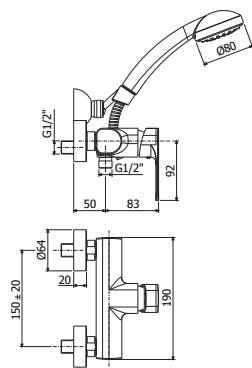
SY 168-168DCR Miscelatore doccia con/senza set doccia Wall mounted shower mixer with/without shower set
