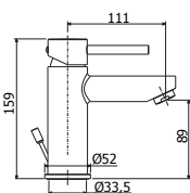
SK 071H-075HCR-EWS Miscelatore lavabo con/ senza scarico, con cartuccia ENERGY & WATER SAVING Wash basin mixer with/ without pop up waste, with ENERGY & WATER SAVING cartridge
