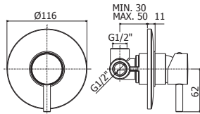
BI 010-011CR Miscelatore incasso doccia / Piastra Ø116 e 110 mm corpo incasso incluso Concealed shower mixer / Wall plate Ø116 and 110 mm concealed body included
