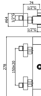
LEQ 269CR Miscelatore termostatico doccia attacco 1/2" x 1/2" con deviatore Thermostatic shower mixer 1/2" x 1/2" connection with diverter
