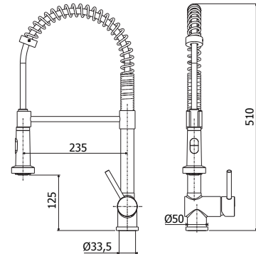
SK 176CR Miscelatore lavello "Professional" con doccetta getto regolabile One-hole sink mixer "Professional" with cylindrical hand-shower with adjustable spray
