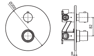
LIQ 013CR Miscelatore termostatico incasso doccia uscite corpo incasso incluso Concealed thermostatic shower mixer concealed body included
