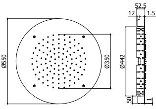
ZSOF 304CR LAS VEGAS Soffione ad incasso "Tondo" in metallo, anticalcare - Ø 550 mm "Round" concealed ceiling metal shower head, antiscaling system - Ø 550 mm
