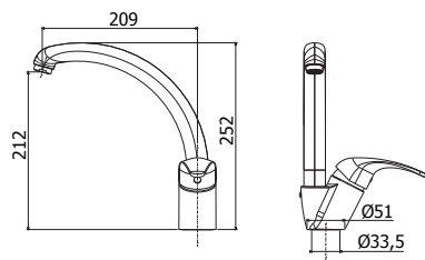
ND 181CR Miscelatore lavello monoforo con canna tubo orientabile One-hole sink mixer with tube swivelling spout
