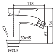
LES 131-131K-135CR Miscelatore bidet con/senza scarico, con scarico Clic-Clac Bidet mixer with/without pop up waste, with Clic-Clac press top waste
