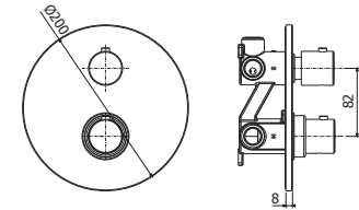
LIQ 018CR Miscelatore termostatico incasso 2 uscite corpo incasso incluso Concealed thermostatic 2 outlets concealed body included
