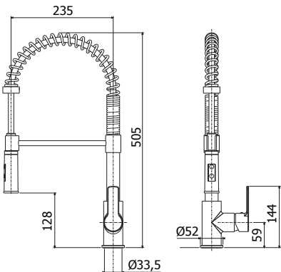
RED 179CR Miscelatore lavello "Professional" con doccia estraibile (2 getti) e canna orientabile One-hole "Professional" sink mixer with pull-out hand-shower (two-spray) and swivelling spout
