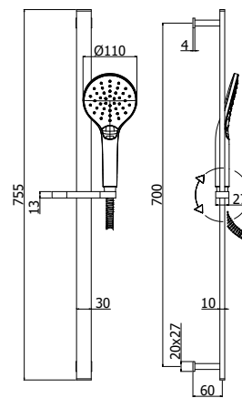
ZSAL 147C RAG CITY SOFIA Saliscendi City Sofia con doccia (2 getti) in ABS City Sofia sliding rail with (2-spray functions) ABS hand-shower
