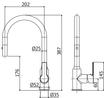
RED 285CR Miscelatore lavello monoforo con doccia estraibile (2 getti) e canna tonda orientabile One-hole sink mixer with pull-out hand-shower (two-spray) and round swivelling spout
