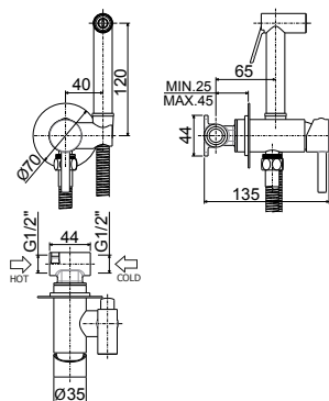
ZDUP 110 - 125CR TWEET ROUND MIX- TWEET PLUS MIX Set bidet incasso con miscelatore, doccia 2 getti Concealed bidet set with mixer, two-spray hand shower
