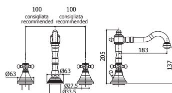
FBLV 052-055 Batteria lavabo con/ senza scarico Three-hole wash basin mixer with/ wi- thout pop up waste
