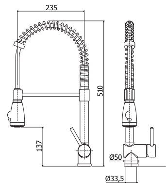
SK 178CR Miscelatore lavello "Professional" con doccetta Lux 2 getti One-hole sink mixer "Professional" with two-spray luxury hand-shower
