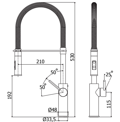
LIG 179CRNO - LIG 179CR Miscelatore lavello monoforo con canna orientabile Professional One-hole sink mixer with swivelling spout Professional
