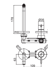
LIG 105-104-106CR70 Miscelatore incasso con bocca erogazione a muro 178 mm / 123 mm / 248 mm corpo incasso incluso Concealed wash basin mixer with wall spout 178 mm / 123 mm / 248 mm concealed body included
