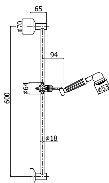
ZSAL 010CR KLIPPER Saliscendi Klipper con doccia (monogetto) in metallo Klipper sliding rail with (single- spray) metal hand-shower
