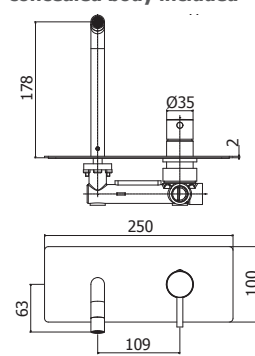
SK 105-104-106CR Miscelatore incasso con bocca erogazione a muro 178 mm / 123 mm / 248 mm corpo incasso incluso Concealed wash basin mixer with wall spout 178 mm / 123 mm / 248 mm concealed body included
