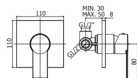
TA 010CR Miscelatore incasso doccia corpo incasso incluso Concealed shower mixer concealed body included
