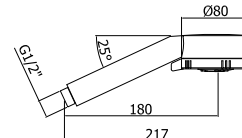
ZDOC 070CR MAJORCA Doccia Majorca (3 getti) in ABS Ø80 mm Majorca (3-spray functions) ABS hand-shower Ø80 mm
