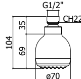
ZSOF 031CR ALABAMA Soffione "Alabama" in ABS, anticalcare Ø 70 mm "Alabama" ABS shower head, antiscala system - Ø 70 mm
