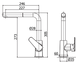
SY 185CR Miscelatore lavello monoforo con doccia estraibile (monogetto) e canna tonda orientabile One-hole sink mixer with pull-out hand-shower (single-spray) and round swivelling spout
