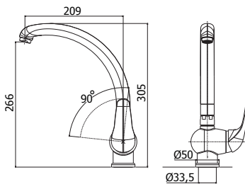
DU 181CR Miscelatore lavello monoforo con canna tubo orientabile One-hole sink mixer with tube swivelling spout
