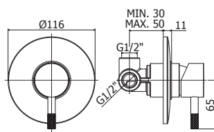
JL 010-010..70-011CR Miscelatore incasso doccia / Piastra Ø116, 70 e 110 mm corpo incasso incluso Concealed shower mixer / Wall plate Ø116, 70 and 110 mm concealed body included
