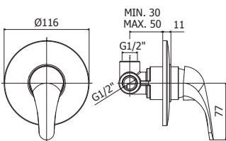
APM3 010CR Miscelatore incasso doccia corpo incasso incluso Concealed shower mixer concealed body included
