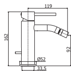
FOX 131- 131K -135CR Miscelatore bidet con/ senza scarico, con scarico Clic-Clac Bidet mixer with/ without pop up waste, with Clic-Clac press top waste
