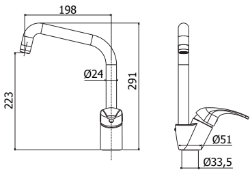
ND 180CR Miscelatore lavello monoforo con canna tubo orientabile One-hole sink mixer with tube swivelling spout
