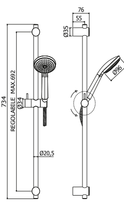
ZSAL 181CR LANCE Plus Saliscendi Lance Plus con doccia (monogetto) in ABS Lance Plus sliding rail with (single- spray) ABS hand-shower
