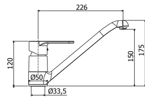
GR 182CR Miscelatore lavello monoforo con canna fusa orientabile One-hole sink mixer with swivelling cast spout
