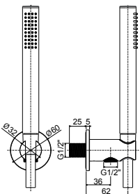
ZDUP 130AC INOX Set doccia incasso tondo con presa acqua incorporata Round concealed shower set with build-in water inlet
