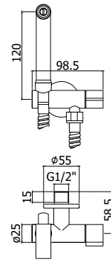
ZDUP 109 - 124CR TWEET ROUND - TWEET PLUS Set bidet incasso con rubinetto solo acqua fredda, doccia 2 getti Concealed bidet set with tap for cold water only, two-spray hand shower
