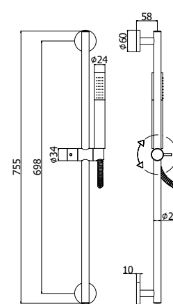
ZSAL 135CRAG LIFE Saliscendi Life con doccia (monogetto) in metallo Life sliding rail with (single-spray) metal hand-shower
