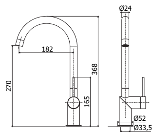
INOX 180AC Miscelatore lavello monoforo con canna orientabile con canna tubo One-hole sink mixer with swivelling spout with tube spout
