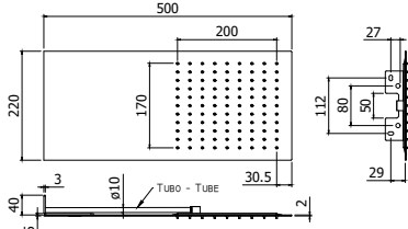
ZSOF 117CR SLIM Soffione "Slim" in metallo, anticalcare - 500x220 mm "Slim" metal shower head, antiscaling system - 500x220 mm
