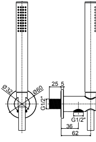
ZDUP 130AC INOX Set doccia incasso tondo con presa acqua incorporata Round concealed shower set with build-in water inlet
