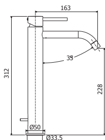
LIG 081-081K-085CR Miscelatore lavabo prolungato con/senza scarico, con scarico Clic-Clac Tall wash basin mixer with/without pop up waste, with Clic-Clac press top waste
