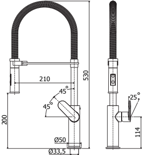
CA 179CR- CA 179CRNO Miscelatore lavello "Professional" con doccia estraibile (2 getti) e canna orientabile One-hole "Professional" sink mixer with pull-out hand-shower (two-spray) and swivelling spout
