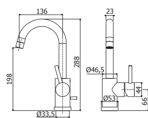
BI 078-077CR Miscelatore lavabo con canna orientabile con/ senza scarico Wash basin mixer with swivelling spout with/ without pop up waste
