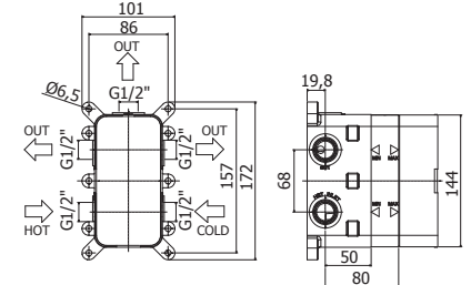
PBOX 003/004 Set incasso universale per miscelatori doccia 2 o 3 vie Universal Concealed Box for mixers 2 or 3 outlet
