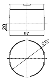
PBOX 005 Set incasso universale per miscelatori VASCA/LAVABO FREESTANDING Universal Concealed Box for Free-standing bath/shower mixer
