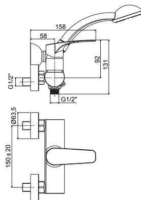
LM 168-168DCR Miscelatore doccia attacco 1/2" con/senza set doccia Shower mixer 1/2" connection with/without shower set
