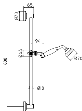
ZSAL 070CR BELINDA Saliscendi Belinda con doccia (monogetto) in metallo Belinda sliding rail with (single- spray) metal hand-shower
