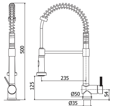
FOX 176CR Miscelatore lavello "Professional" con doccetta getto regolabile One-hole sink mixer "Professional" with cylindrical hand-shower with adjustable spray
