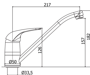
DU 182TCR Miscelatore lavello monoforo con canna tubo orientabile One-hole sink mixer with tube swivelling spout
