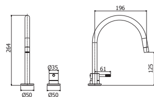
JL 051-051KCR Batteria lavabo con/senza scarico 2-hole wash basin mixer with/without pop up waste
