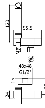
ZDUP 111CR TWEET SQUARE Set bidet incasso con rubinetto solo acqua fredda Concealed bidet set with tap for cold water only
