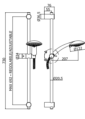
ZSAL 118CR PRESTIGE Saliscendi Prestige con doccia (4 getti) in ABS Prestige sliding rail with (4-spray functions) ABS hand-shower
