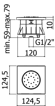
ZSOF 121CR Soffione quadro in ABS, anticalcare, con getto orientabile - 124.5x124.5 mm Square ABS body jet, antiscaling system, with swivelling spray - 124.5x124.5 mm
