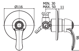
FA 010-011CR Miscelatore incasso doccia / Piastra Ø116 e Ø110 mm corpo incasso incluso Concealed shower mixer / Wall plate Ø116 and Ø110 mm concealed body included
