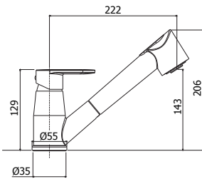
CA 183CR Miscelatore lavello con doccia estraibile (2 getti) e canna orientabile One-hole sink mixer with pull-out hand- shower (two-spray) and swivelling spout
