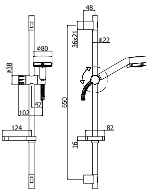
ZSAL 110CR MANILA Saliscendi Manila con doccia (3 getti) in ABS Manila sliding rail with (3-spray functions) ABS hand-shower
