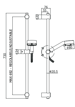
ZSAL 105CR MAJORCA Saliscendi Majorca con doccia (3 getti) in ABS Majorca sliding rail with (3-spray functions) ABS hand-shower
