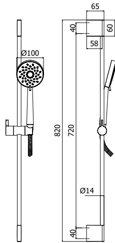
ZSAL 212CR LUNA TOP Saliscendi Luna Top con doccia (3 getti) in ABS Luna Top sliding rail with (3-spray functions) ABS hand-shower
