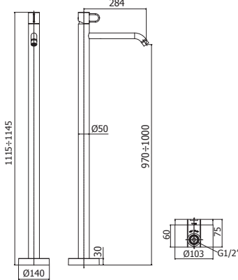
JKBOX 031CR Miscelatore lavabo a pavimento Free-standing basin mixer
