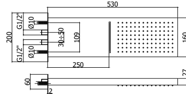
ZSOF 099CR CASCADE Soffione "Cascade" (2 getti) in metallo, anticalcare - 530x160 mm (2-spray) "Cascade" metal shower head, antiscaling system - 530x160 mm
