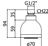
ZSOF 032CR OREGON Soffione "Oregon" in ABS, anticalcare Ø 70 mm "Oregon" ABS shower head, antiscala system - Ø 70 mm
