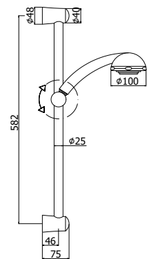
ZSAL 064CR ISCHIA Saliscendi Ischia con doccia (3 getti) in ABS Ischia sliding rail with (3-spray functions) ABS hand-shower
