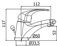
ND 071-075CR Miscelatore lavabo con/ senza scarico Wash basin mixer with/ without pop up waste
