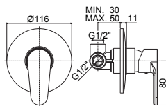
GR 010CR Miscelatore incasso doccia corpo incasso incluso Concealed shower mixer concealed body included
