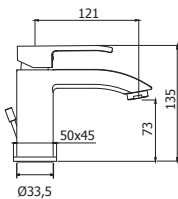
LES 071-071K-075CR Miscelatore lavabo con/senza scarico, con scarico Clic-Clac Wash basin mixer with/without pop up waste, with Clic-Clac press top waste
