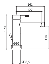
JL 071-071K-075CR Miscelatore lavabo con/senza scarico, con scarico Clic-Clac Wash basin mixer with/without pop up waste, with Clic-Clac press top waste
