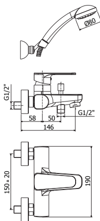
SY 022-023-024-026CR Miscelatore vasca/doccia con/senza set doccia, con supporto Stick, con supporto fisso in ABS Bath/shower mixer with/without shower set, with Stick wall bracket, with ABS fixed wall bracket
