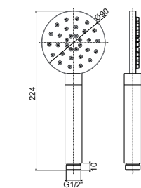
ZDOC 133AC INOX Doccia Soft (monogetto) in acciaio Ø90mm Soft (single-spray) steel hand-shower Ø90mm
