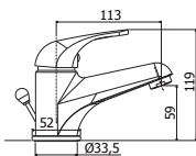
APM3 071-075CR Miscelatore lavabo con/ senza scarico con attacco catenella Wash basin mixer with/ without pop up waste with chain holder
