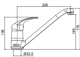
ND 182CR Miscelatore lavello monoforo canna fusa orientabile One-hole sink mixer with swivelling cast spout
