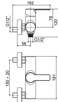
RED 168-168DCR Miscelatore doccia con/senza set doccia Wall mounted shower mixer with/without shower set
