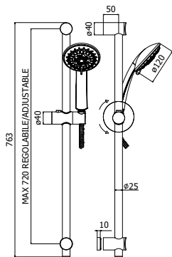
ZSAL 132CR PANAMA Saliscendi Prince con doccia (4 getti) in ABS Prince sliding rail with (4-spray functions) ABS hand-shower
