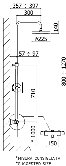
ZCOL 633LIQCR MINI BIRILLO CONFORT Colonna doccia con miscelatore termostatico - COULD TOUCH Shower column with thermostatic mixer - COULD TOUCH
