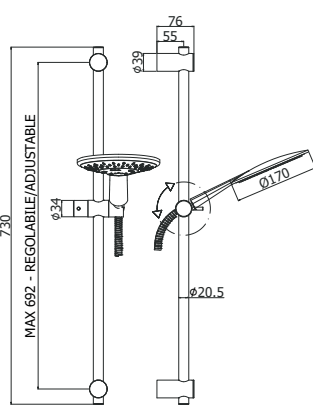
ZSAL 196CR ODEON Saliscendi Odeon con doccia (monogetto) in ABS Odeon sliding rail with (single- spray) ABS hand-shower
