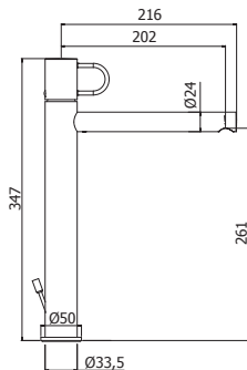
JK 081-071K-085CR Miscelatore lavabo prolungato con/senza scarico, con scarico Clic-Clac Tall wash basin mixer with/without pop up waste, with Clic-Clac press top waste
