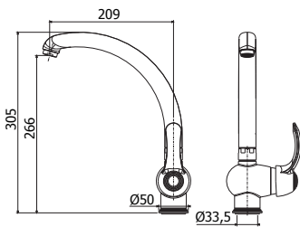
FA 181CR Miscelatore lavello laterale canna alta orientabile One-hole sink mixer high swivelling spout
