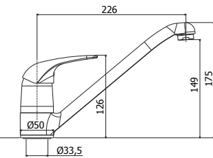
DU 182CR Miscelatore lavello monoforo canna fusa orientabile One-hole sink mixer with swivelling cast spout
