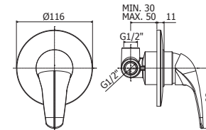
DU 010CR Miscelatore incasso doccia corpo incasso incluso Concealed shower mixer concealed body included
