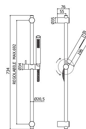
ZSAL 150CR STICK NEW Saliscendi Stick new con doccia (monogetto) in ABS Stick new sliding rail with (single- spray) ABS hand-shower
