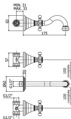
FBLV 003-008CR Batteria lavabo incasso con bocca a muro 175 / 245 mm Three-hole concealed wash basin mixer with wall spout 175 / 245 mm
