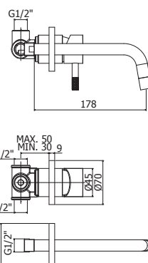
JL 006-007CR70 Miscelatore incasso con bocca erogazione a muro 175 mm / 245 mm corpo incasso incluso Concealed two-hole basin mixer with wall spout 175 mm / 245 mm concealed body included
