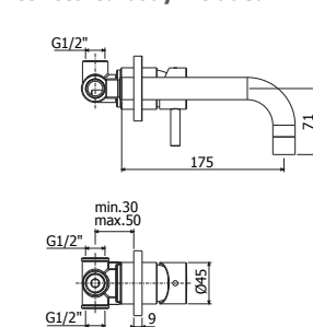
SK 006-007CR70 Miscelatore incasso con bocca erogazione a muro 175 mm / 245 mm corpo incasso incluso Concealed two-hole basin mixer with wall spout 175 mm / 245 mm concealed body included
