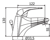
DU 071-075CR Miscelatore lavabo con/senza scarico Wash basin mixer with/without pop up waste
