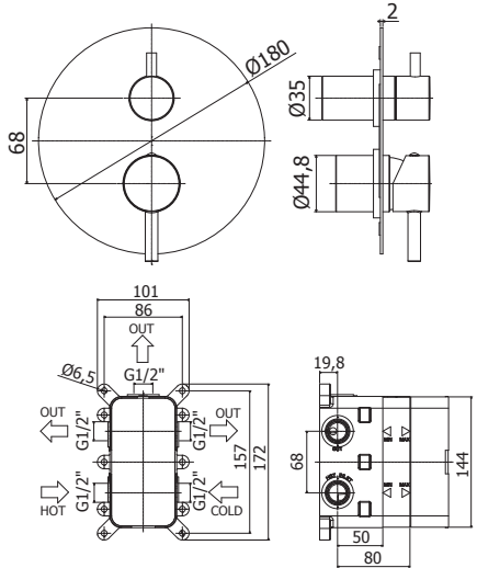
PBOX 003/004 Set incasso universale per miscelatori doccia 2 o 3 vie Universal Concealed Box for mixers 2 or 3 outlet
