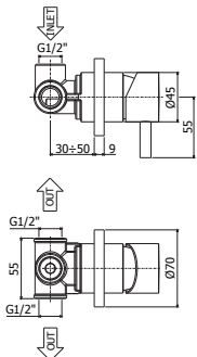
ZDEV 118CR70-LIG Deviatore incasso completo di piastra in metallo Ø 70 corpo incasso incluso Concealed diverter with metal wall plate Ø70 concealed body included
