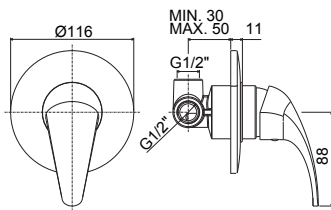
ND 010CR Miscelatore incasso doccia corpo incasso incluso Concealed shower mixer concealed body included
