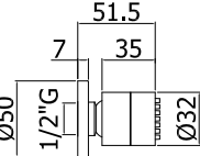
ZSOF 061CR Soffione tondo in metallo, anticalcare - Ø32 mm Round metal body jet, antiscaling system Ø32 mm
