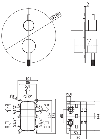
PBOX 003/004 Set incasso universale per miscelatori doccia 2 o 3 vie Universal Concealed Box for mixers 2 or 3 oulet
