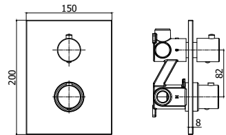
LIQ 518CR Miscelatore termostatico incasso 2 uscite corpo incasso incluso Concealed thermostatic 2 outlets concealed body included
