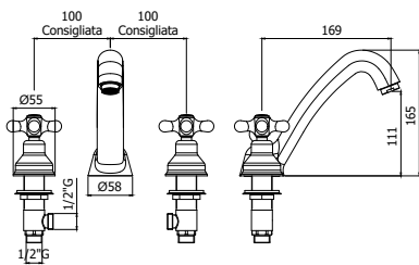
IRV 052-055CR Batteria lavabo con canna fissa con/ senza scarico Three-hole wash basin mixer with fixed spout with/without pop up waste
