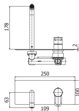
JK 105-104-106CR Miscelatore incasso con bocca erogazione a muro 178 mm / 123 mm / 248 mm corpo incasso incluso Concealed wash basin mixer with wall spout 178 mm / 123 mm / 248 mm concealed body included
