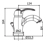
FA 071-075CR Miscelatore lavabo con/ senza scarico Wash basin mixer with/ without pop up waste
