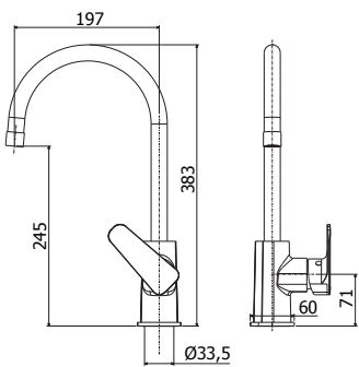
SY 181CR Miscelatore lavello monoforo con canna tonda orientabile One-hole sink mixer with round swivelling spout
