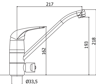
DU 184CR Miscelatore lavello monoforo con canna orientabile e attacco lavastoviglie Tall one-hole sink mixer with swivelling spout and dish-washer machine connection
