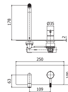
JL 105-104-106CR Miscelatore incasso con bocca erogazione a muro 178 mm / 123 mm / 248 mm corpo incasso incluso Concealed wash basin mixer with wall spout 178 mm / 123 mm / 248 mm concealed body included
