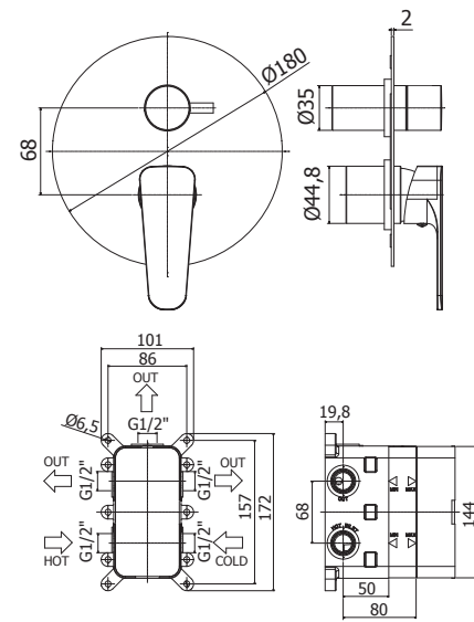
PBOX 003/004 Set incasso universale per miscelatori doccia 2 o 3 vie Universal Concealed Box for mixers 2 or 3 outlet
