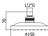
ZSOF 029CR ARIZONA Soffione "Arizona" in ABS, anticalcare Ø 150 mm "Arizona" ABS shower head, antiscala system - Ø150 mm
