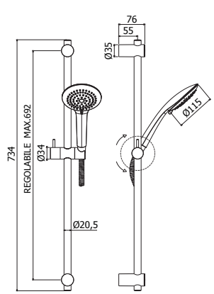
ZSAL 120CR PRINCE Plus Saliscendi Prince Plus con doccia (4 getti) in ABS Prince Plus xsliding rail with (4-spray functions) ABS hand- shower
