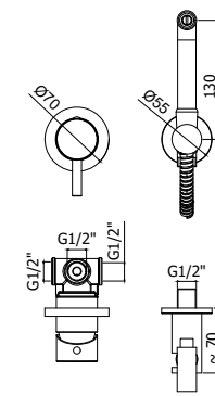
KIT DUP110-125CR TWEET ROUND-TWEET PLUS Set bidet incasso con miscelatore, doccia 2 getti Concealed bidet set with mixer, two- spray hand shower
