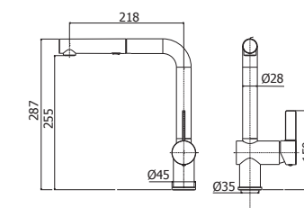
RO 285CR Miscelatore lavello monoforo con doccia estraibile (2 getti) e canna orientabile One-hole sink mixer with pull-out hand-shower (two-spray) and swivelling spout
