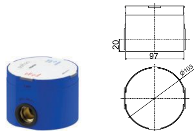
PBOX 005 Set incasso universale per miscelatori VASCA/LAVABO FREESTANDING Universal Concealed Box for Free-standing bath/shower mixer * Da abbinare solo con EL BOX033 To be completed only with EL BOX033
