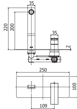
LES 105-104-106CR Miscelatore incasso con bocca erogazio- ne a muro 200 mm / 150 mm / 240 mm corpo incasso incluso Concealed wash basin mixer with wall spout 200 mm / 150 mm / 240 mm concealed body included
