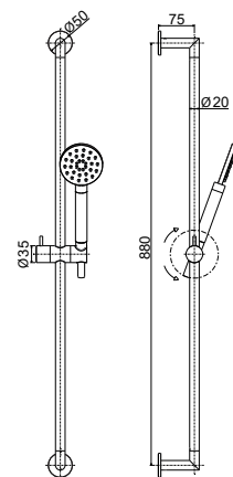
ZSAL 215AC INOX SOFT Saliscendi INOX con doccia e supporto scorrevole INOX sliding rails with hand-shower and slider bracket
