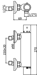
EQS 168-168DCRNEW Miscelatore termostatico doccia attacco 1/2" con senza set doccia Thermostatic shower mixer 1/2" connection with without shower kit
