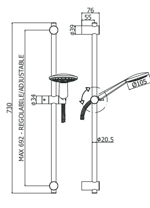
ZSAL 195CR GIADA Saliscendi Giada con doccia (monogetto) in ABS Giada sliding rail with (single- spray) ABS hand-shower
