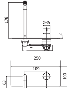
FOX 105-104-106CR Miscelatore incasso con bocca erogazione a muro 178 mm / 123 mm / 248 mm corpo incasso incluso Concealed wash basin mixer with wall spout 178 mm / 123 mm / 248 mm concealed body included
