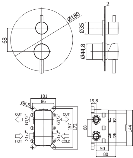
PBOX 003/004 Set incasso universale per miscelatori doccia 2 o 3 vie Universal Concealed Box for mixers 2 or 3 oulet
