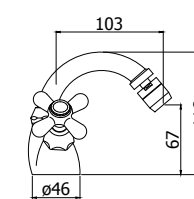
IRV 137-138CR Monoforo bidet con canna orientabile, con/senza scarico One-hole bidet mixer with swivelling spout, with/without pop up waste
