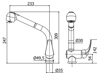
ND 185CR Miscelatore lavello con doccia estraibile (2 getti) e canna orientabile One-hole sink mixer with pull-out hand- shower (two-spray) and swivelling spout
