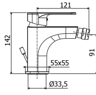
SY 131-131K-135CR Miscelatore bidet con/senza scarico, con scarico Clic-Clac Bidet mixer with/without pop up waste, with Clic-Clac press top waste
