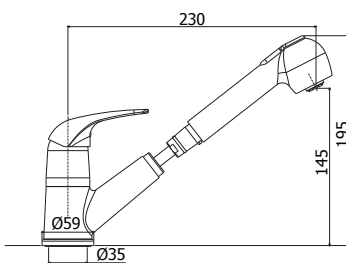
DU 183CR Miscelatore lavello con doccia estaibile (2 getti) e canna tubo orientabile One-hole sink mixer with pull-out hand-shower (two-spray) and swivelling spout
