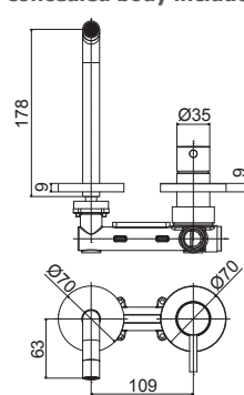
SK 105-104-106CR70 Miscelatore incasso con bocca erogazione a muro 178 mm / 123 mm / 248 mm corpo incasso incluso Concealed wash basin mixer with wall spout 178 mm / 123 mm / 248 mm concealed body included
