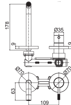
JL 105-104-106CR70 Miscelatore incasso con bocca erogazione a muro 178 mm / 123 mm / 248 mm corpo incasso incluso Concealed wash basin mixer with wall spout 178 mm / 123 mm / 248 mm concealed body included
