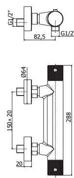
JOQ 168E-168EDCR Miscelatore termostatico doccia attacco 1/2" con/ senza set doccia, con limitatore di portata ECO-STOP Thermostatic shower mixer 1/2" connection with/ without shower kit, with flow reducer ECO-STOP
