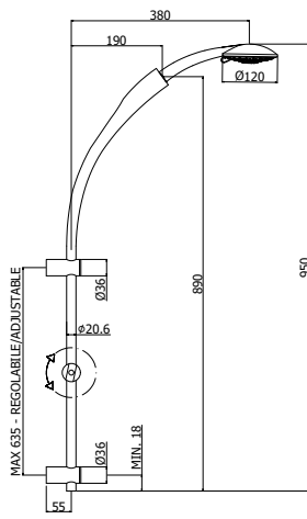
ZSAL 197CR TWIN Saliscendi Twin con doccia (4 getti) in ABS Twin sliding rail with (4-spray functions) ABS hand-shower
