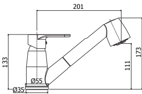
GR 183CR Miscelatore lavello con doccia estraibile (2 getti) e canna tubo orientabile One-hole sink mixer with pull-out hand-shower (two-spray) and swivelling spout
