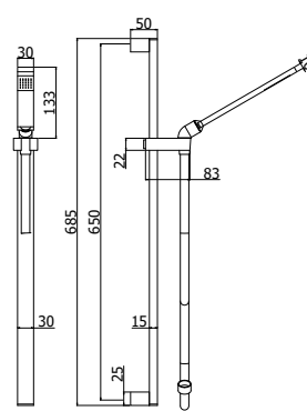
ZSAL 079CR LEVEL Saliscendi Level con doccia (monogetto) in ABS Level sliding rail with (sin- gle-spray) ABS hand-shower
