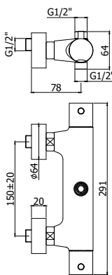
LIQ 169CR Miscelatore termostatico doccia (2 uscite) attacco 1/2" x 1/2" con deviatore Thermostatic shower mixer (2 outlets) 1/2" x 1/2" connection with diverter
