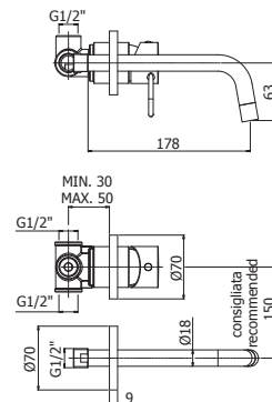
JK 006-007CR70 Miscelatore incasso con bocca erogazione a muro 175 mm / 245 mm corpo incasso incluso Concealed two-hole basin mixer with wall spout 175 mm / 245 mm concealed body included
