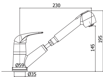
ND 183CR Miscelatore lavello con doccia estraibile (2 getti) e canna tubo orientabile One-hole sink mixer with pull-out hand- shower (two-spray) and swivelling spout
