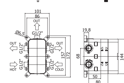
PBOX 003/004 Set incasso universale per miscelatori doccia 2 o 3 vie Universal Concealed Box for mixers 2 or 3 outlet
