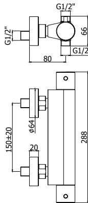
LIQ 469CR COLD TOUCH - ECOSTOP Miscelatore termostatico doccia (2 uscite) attacco 1/2" x 1/2" con cartuccia deviatore Thermostatic shower mixer (2 outlets) 1/2" x 1/2" connection with diverter cartridge
