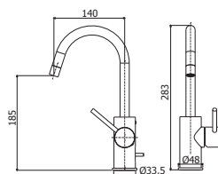
LIG 078-077CR Miscelatore lavabo con canna orientabile con/senza scarico Wash basin mixer with swivelling spout with/without pop up waste
