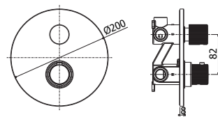
JOQ 013CR Miscelatore termostatico incasso doccia corpo incasso incluso Concealed thermostatic shower mixer concealed body included
