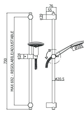
ZSAL 194CR BRIO Saliscendi Brio con doccia (4 getti) in ABS Brio sliding rail with (4-spray functions) ABS hand-shower
