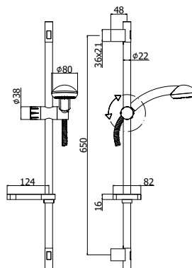
ZSAL 112CR TRIESTE Saliscendi Trieste con doccia (monogetto) in ABS Trieste sliding rail with (single- spray) ABS hand-shower
