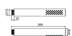
ZDOC 129CR BIRILLO PLUS Doccia Birillo Plus (monogetto) in ABS Birillo Plus(single-spray) ABS hand-shower
