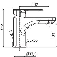
SY 071-075CR-EWS Miscelatore lavabo con/senza scarico, con cartuccia ENERGY & WATER SAVING Wash basin mixer with/without pop up waste, with ENERGY & WATER SAVING cartridge
