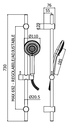
ZSAL 211CR GINEVRA Saliscendi Ginevra con doccia (3 getti) in ABS Ginevra sliding rail with (3-spray functions) ABS hand-shower
