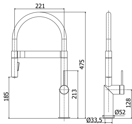
INOX 179AC Miscelatore lavello monoforo con canna orientabile Professional One-hole sink mixer with swivelling spout Professional
