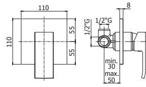
LES 010CR Miscelatore incasso doccia corpo incasso incluso Concealed shower mixer concealed body included
