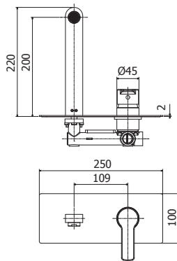
RED 105-104-106CR Miscelatore incasso con bocca erogazione a muro 200 mm / 150 mm / 240 mm corpo incasso incluso Concealed wash basin mixer with wall spout 200 mm / 150 mm / 240 mm concealed body included
