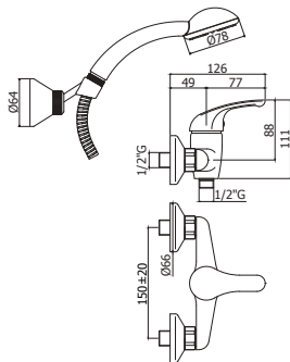
APM3 168-168DCR Miscelatore doccia con/ senza set doccia Wall mounted shower mixer with/ without shower set
