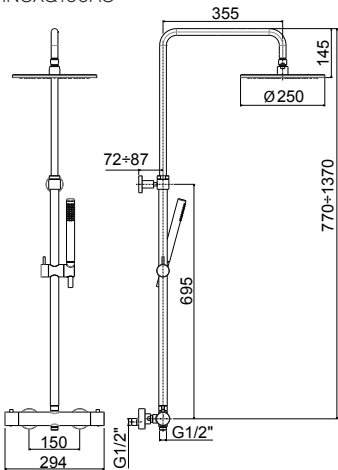
ZCOL 503AC INOX TECH Colonna doccia con miscelatore termostatico INOXQ169AC Shower column with thermostatic mixer INOXQ169AC
