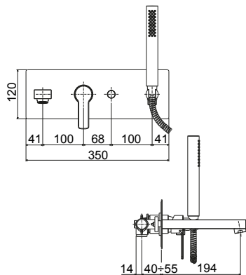
RED 001CR Miscelatore vasca incasso completo di deviatore, bocca e set doccia corpo incasso incluso Concealed bath/shower mixer complete with diverter, spout and shower kit concealed body included
