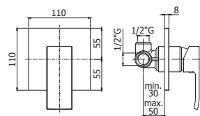
EL 010CR Miscelatore incasso doccia corpo incasso incluso Concealed shower mixer concealed body included
