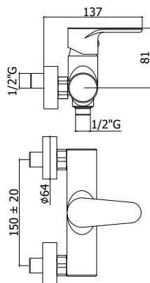
GR 168-168DCR Miscelatore doccia con/ senza set doccia Wall mounted shower mixer with/ without shower set
