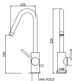
LIG 978-977CR Miscelatore lavabo con canna orientabile con/senza scarico Wash basin mixer with swivelling spout with/without pop up waste
