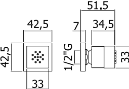
ZSOF 062CR Soffione quadro in metallo, anticalcare - 33x33 mm Square metal body jet, antiscaling system - 33x33 mm
