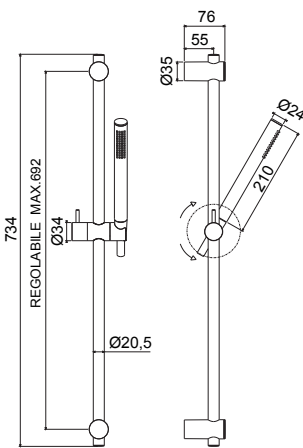
ZSAL 122NO MASTER Saliscendi Master con doccia e supporto scorrevole Master sliding rail with hand- shower and slider bracket
