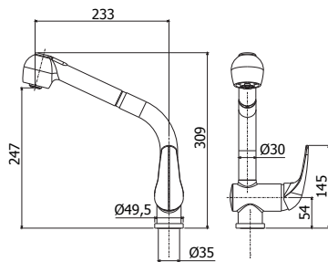
DU 185CR Miscelatore lavello con doccia estaibile (2 getti) e canna orientabile One-hole sink mixer with pull-out hand-shower (two-spray) and swivelling spout
