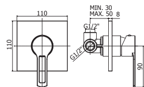
RIN 010CR Miscelatore incasso doccia corpo incasso incluso Concealed shower mixer concealed body included
