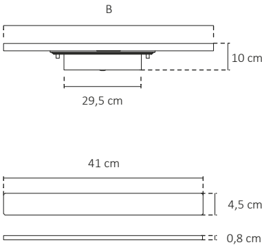
Válvula e grelha incluídas / Valve and grille included
